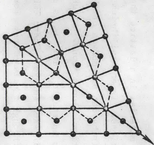
(a) CROSS SECTION OF A TWIN IN BCC IRON AS VIEWED ON THE (110) PLANE
